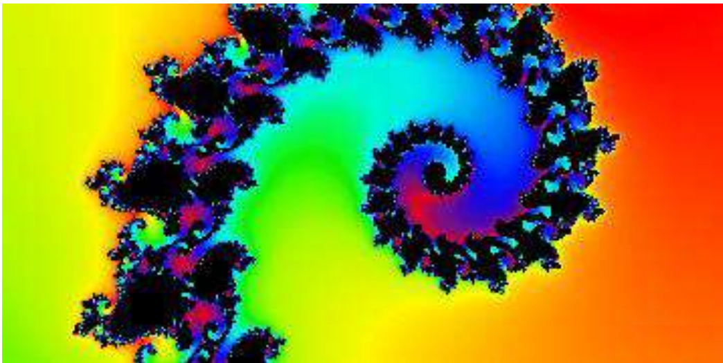
Figure: Fractals
