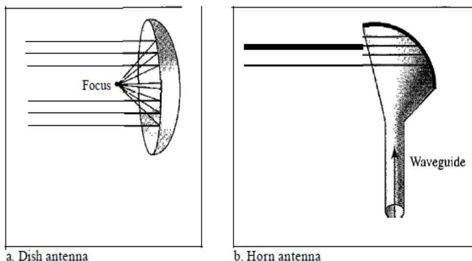
Figure 7.21 Unidirectional antennas
