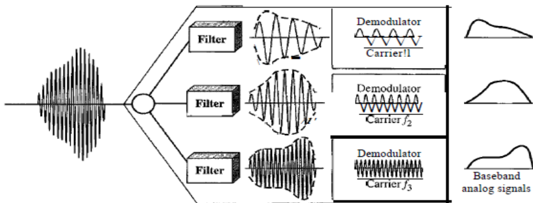
Figure 6.5 FDM demultiplexing example
