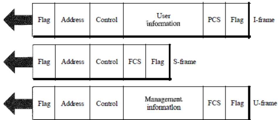
Figure 11.27 HDLC frames
