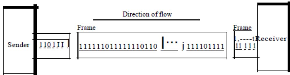
Figure 4.35 Synchronous transmission
