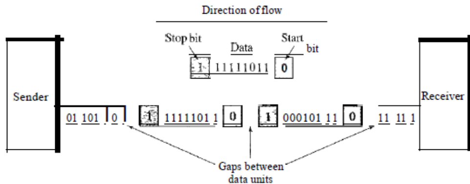
Figure 4.34 Asynchronous transmission
