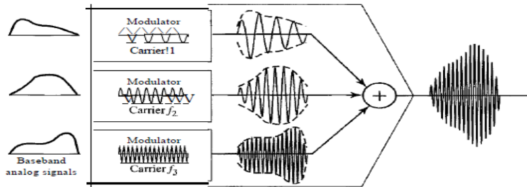
Figure 6.4 FDM process
