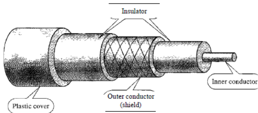
Figure 7.7 Coaxial cable
