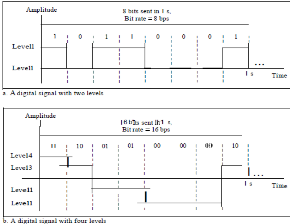
b. A digital signal with four levels
