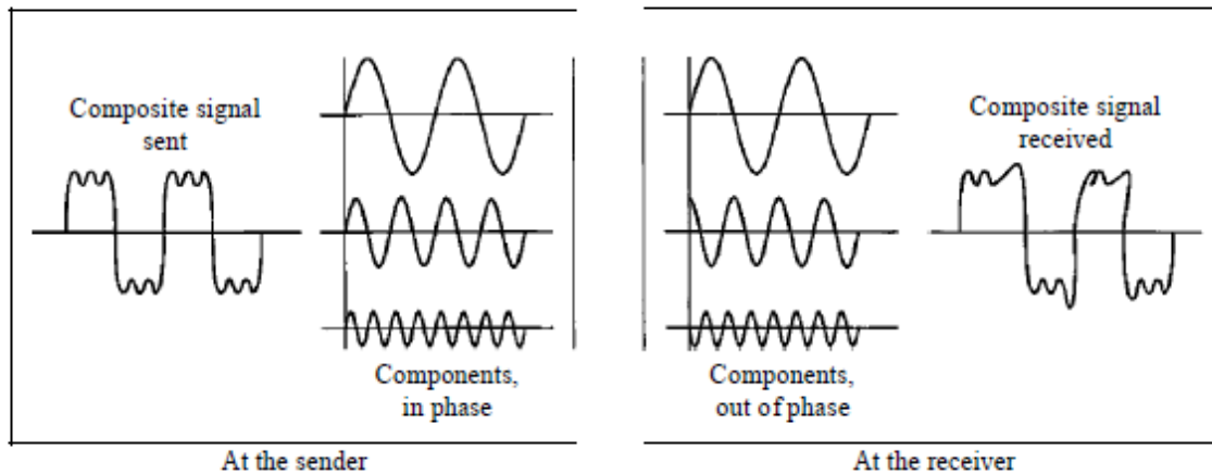
Figure 3.28 Distortion
