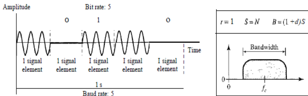
Figure 5.3 Binary amplitude shift keying
