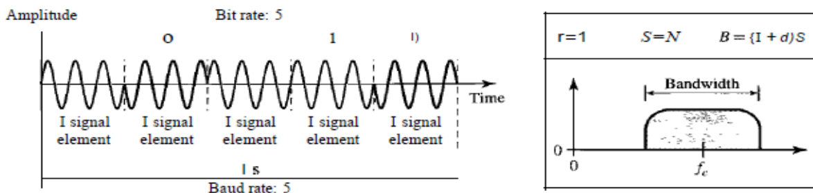
Figure 5.9 Binary phase shift keying
