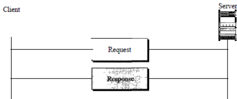
Figure 27.12 HTTP transaction
