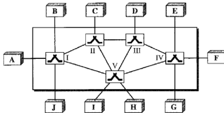
Figure 8.1 Switched network
