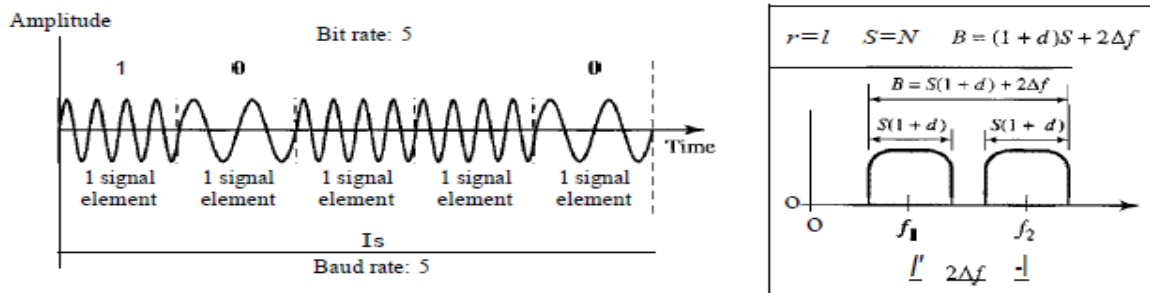
Figure 5.6 Binary frequency shift keying
