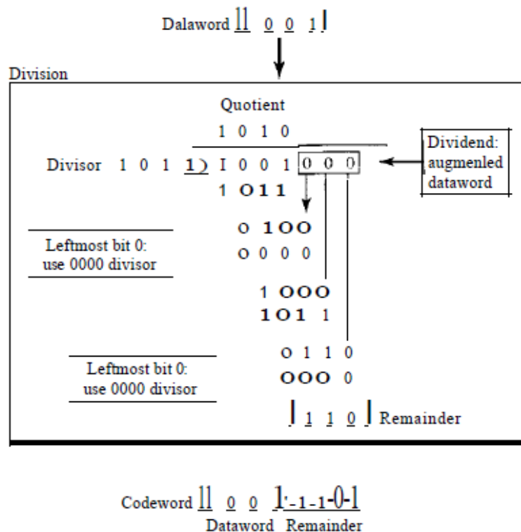
Figure 10.15 Division in CRC encoder
